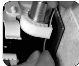
7. Connect wiring. Remove cover and connect green power adapter wire to green power receptacle inside SSPS and secure into wire harness.
